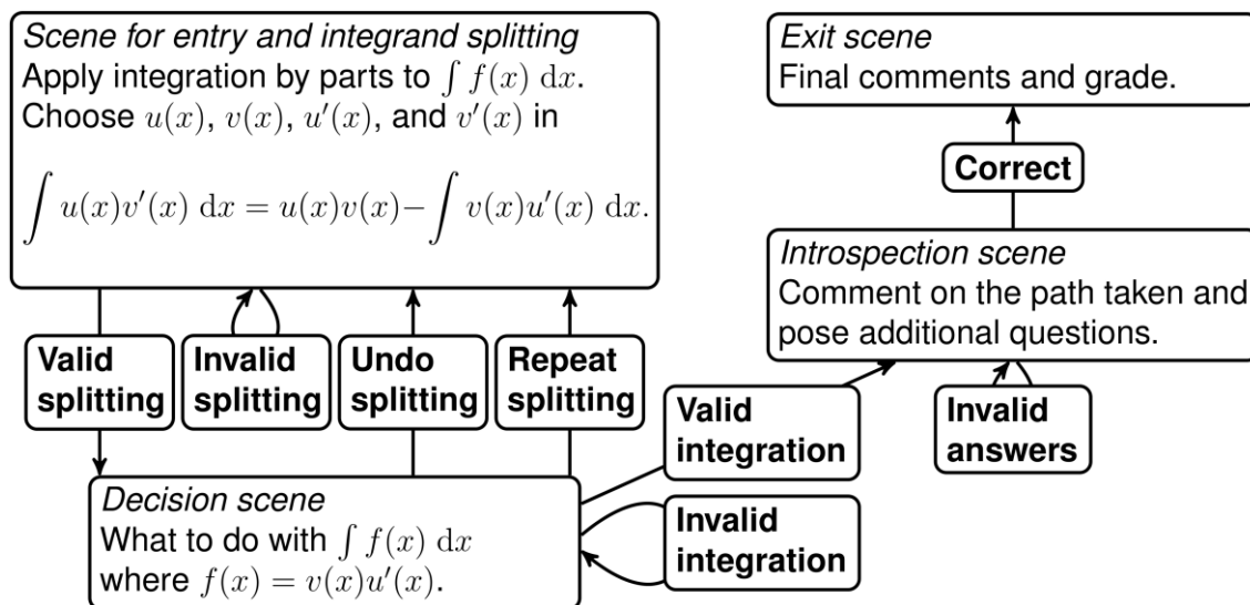
Figure 1. The state transitions of the example question having four scenes.
